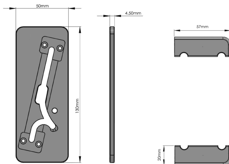
Ground plate
